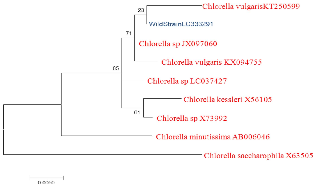
Fig. 1. The Relationship between The Sequences of accession number LC333291 and 8 Accession numbers from gene bank. The Phylogenetic tree was constructed by applying the algorithms maximum likelihood.
